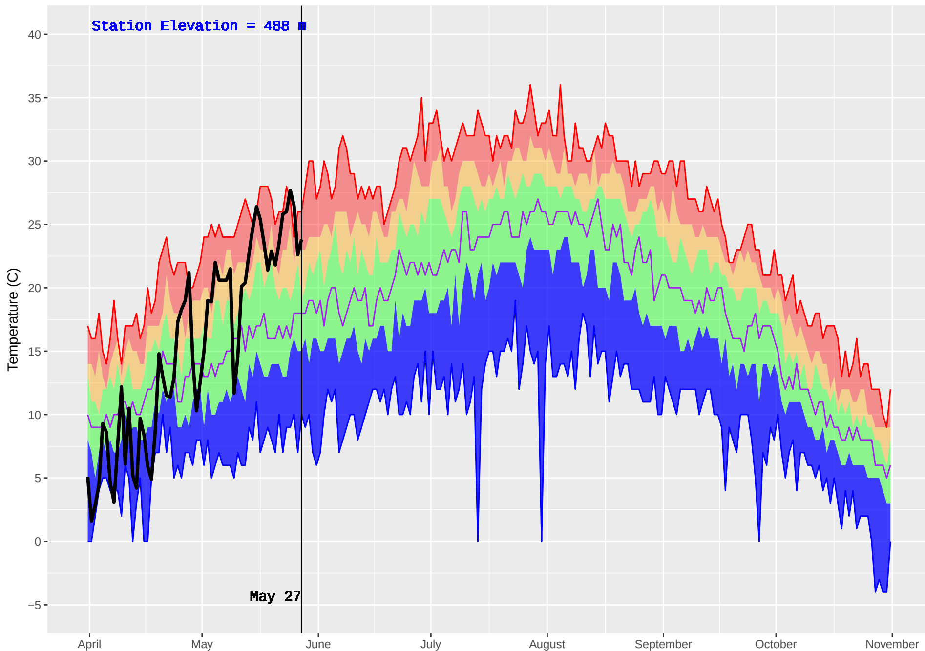
MABEL LAKE 2 (362) : Historical (1987–2016) and Current (2018) Noon Temperature
