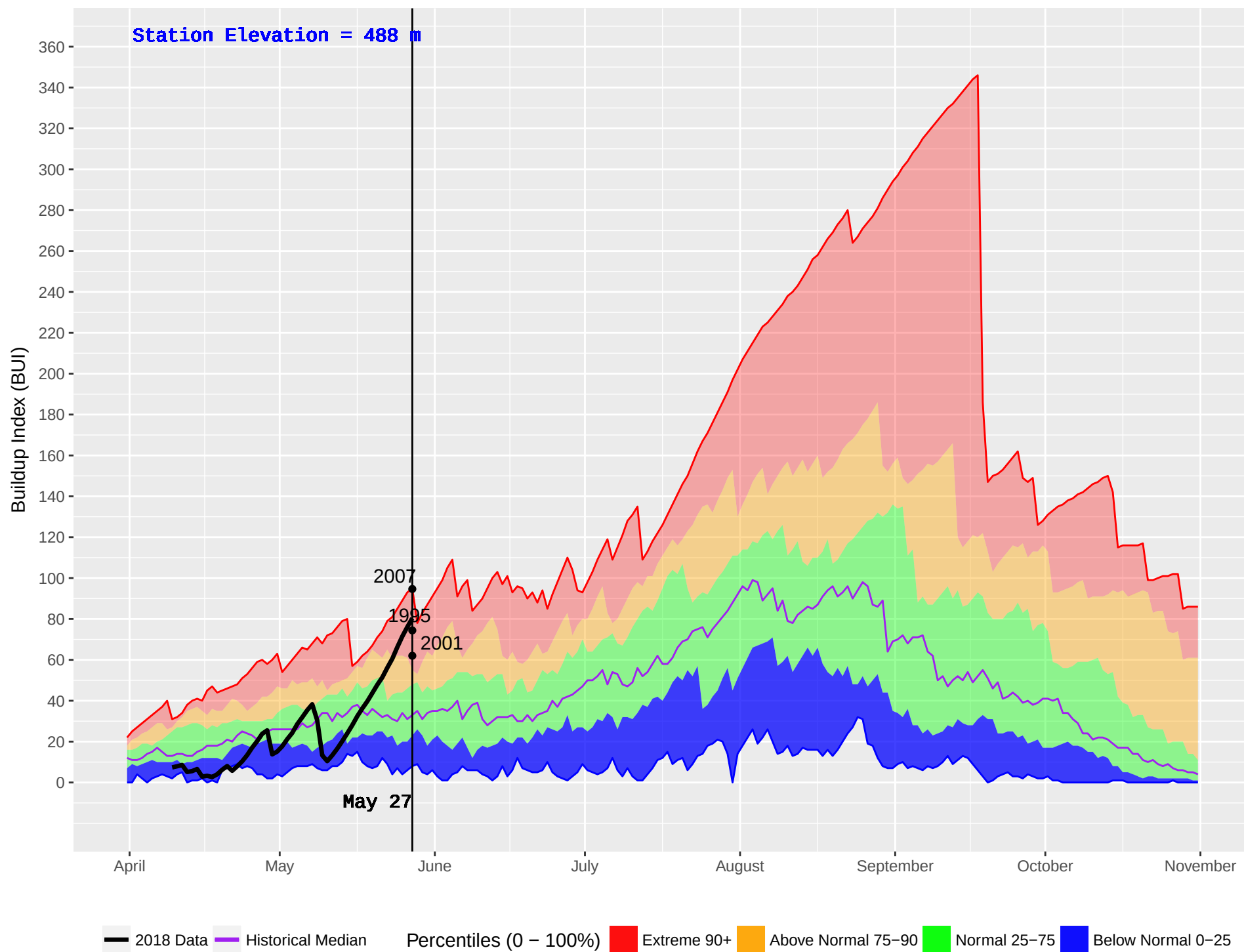
MABEL LAKE 2 (362) : Historical (1987–2016) and Current (2018) Noon Buildup Index (BUI)
