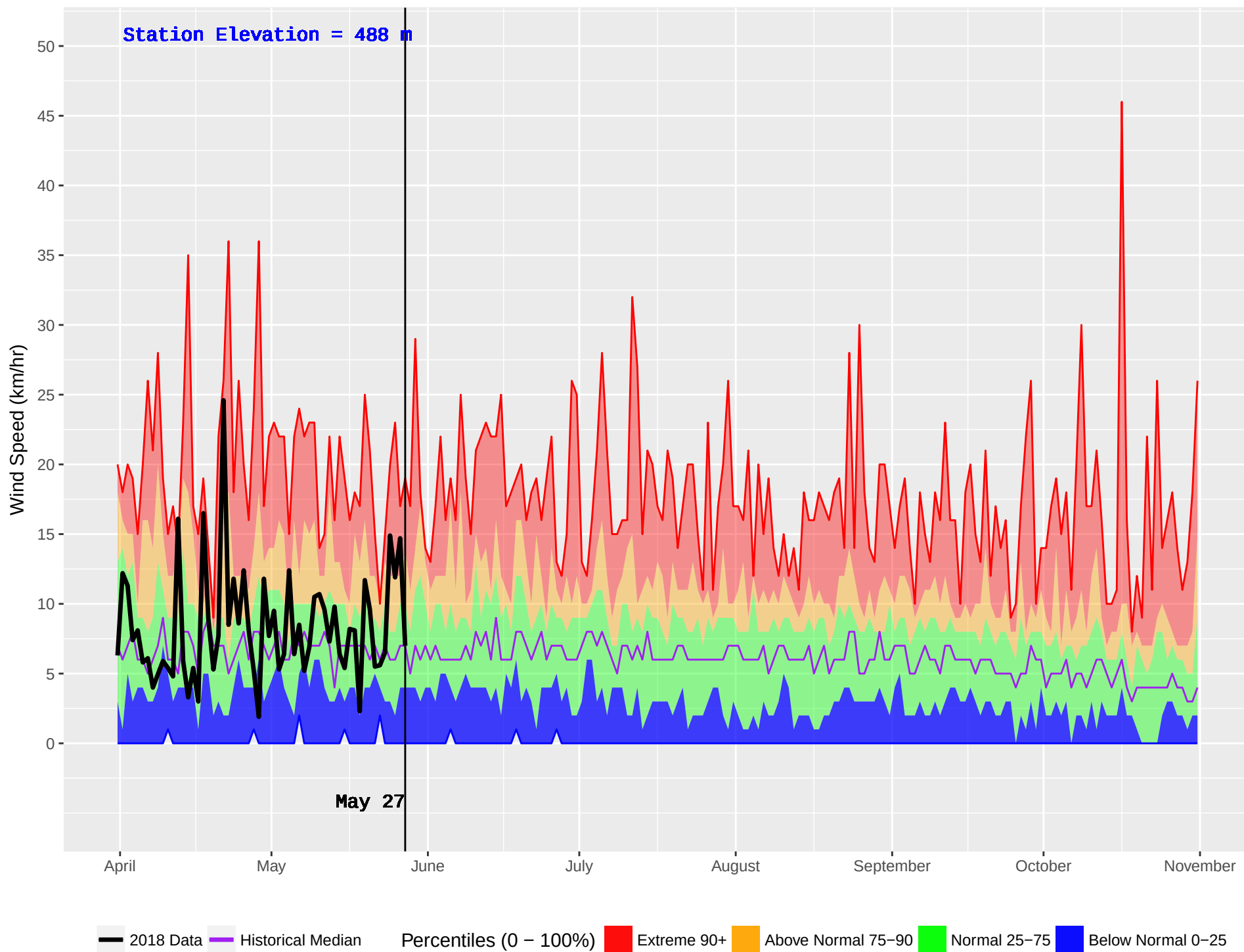
MABEL LAKE 2 (362) : Historical (1987–2016) and Current (2018) Noon Wind Speed
