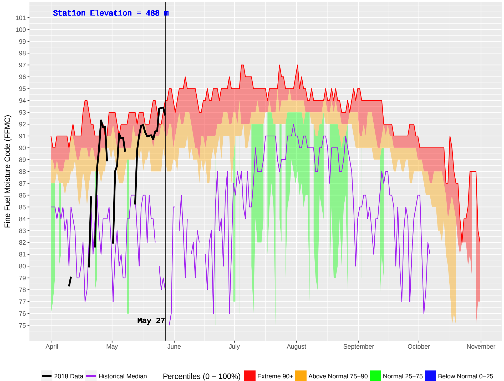
MABEL LAKE 2 (362) : Historical (1987–2016) and Current (2018) Noon Fine Fuel Moisture Code (FFMC)
