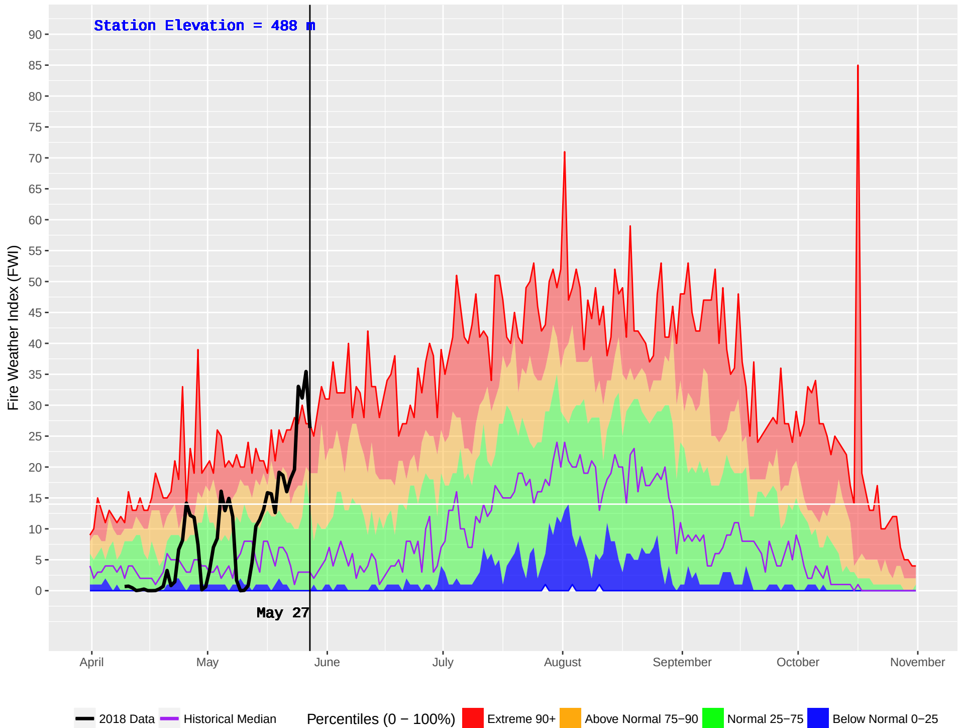
MABEL LAKE 2 (362) : Historical (1987–2016) and Current (2018) Noon Fire Weather Index (FWI)
