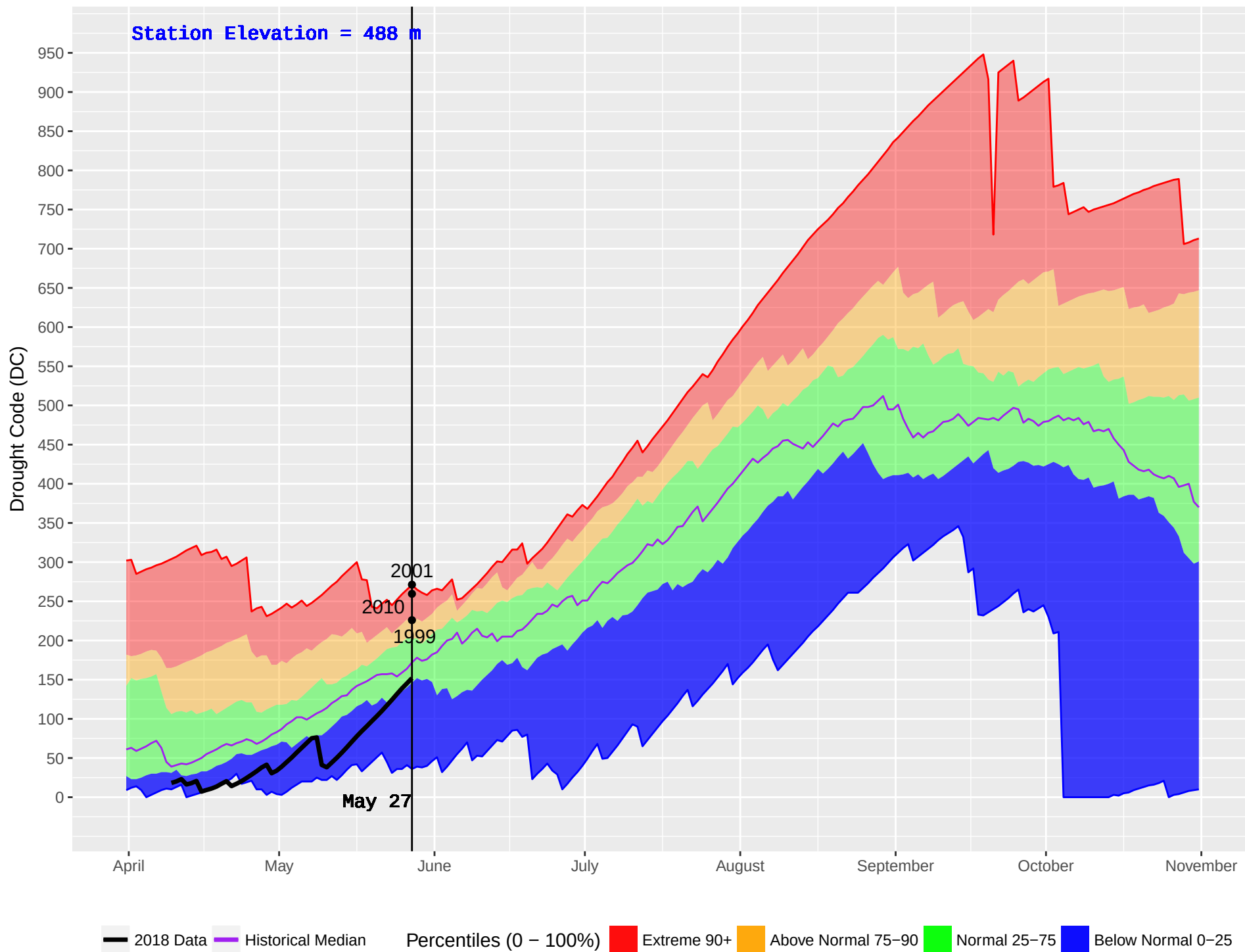
MABEL LAKE 2 (362) : Historical (1987–2016) and Current (2018) Noon Drought Code (DC)
