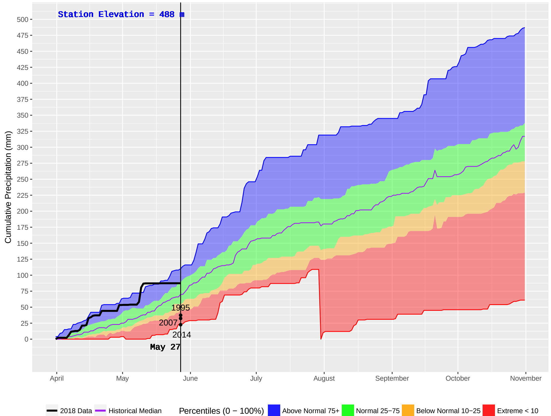
MABEL LAKE 2 (362) : Historical (1987–2016) and Current (2018) Noon Cumulative Precipitation
