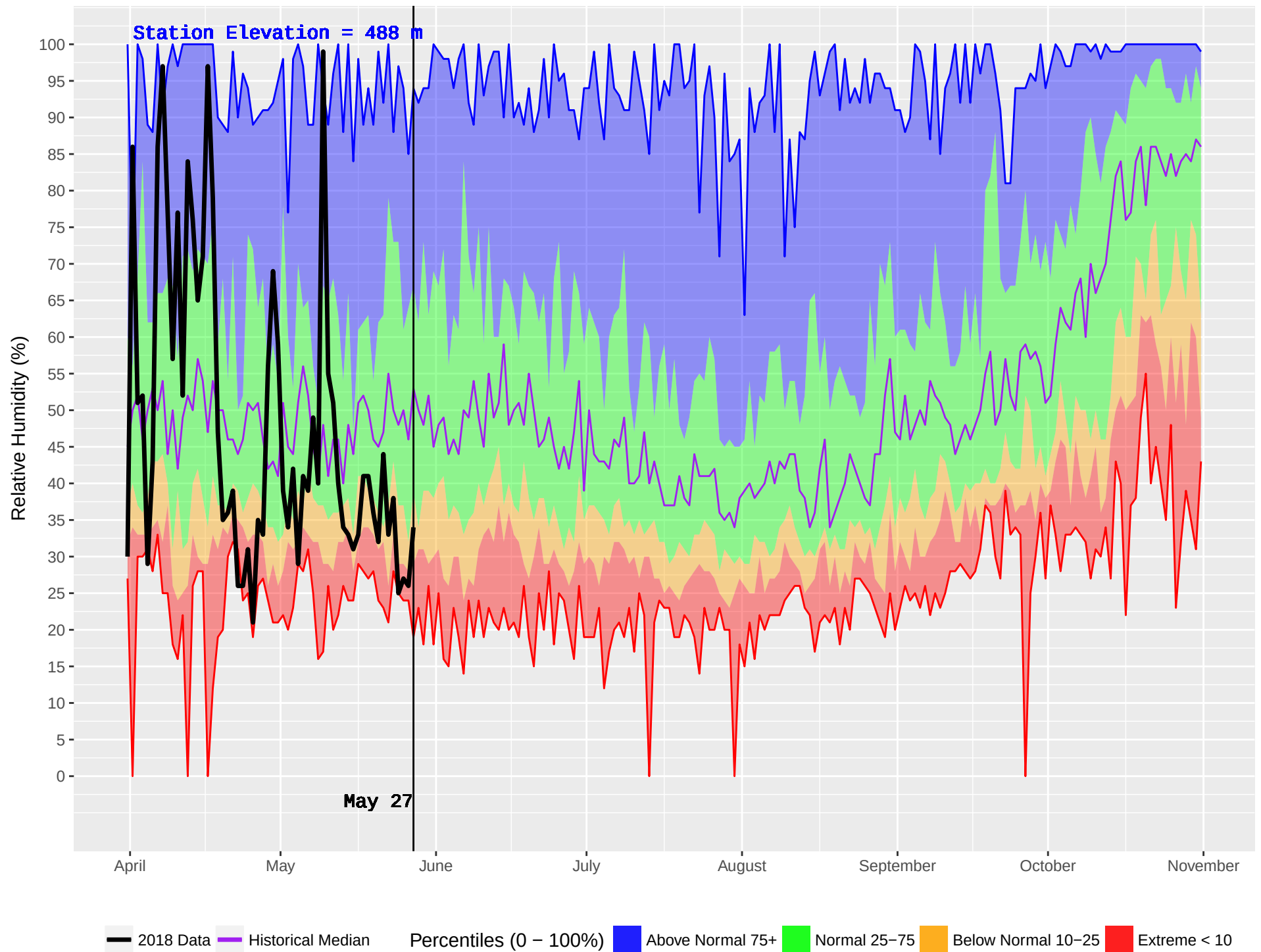
MABEL LAKE 2 (362) : Historical (1987–2016) and Current (2018) Noon Relative Humidity
