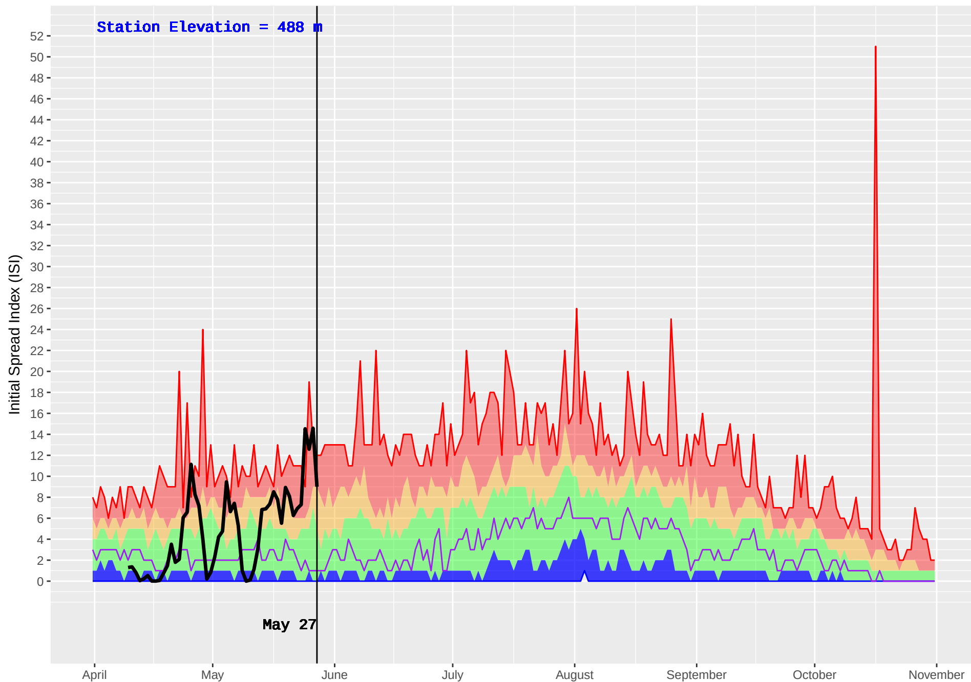
MABEL LAKE 2 (362) : Historical (1987–2016) and Current (2018) Noon Initial Spread Index (ISI)
