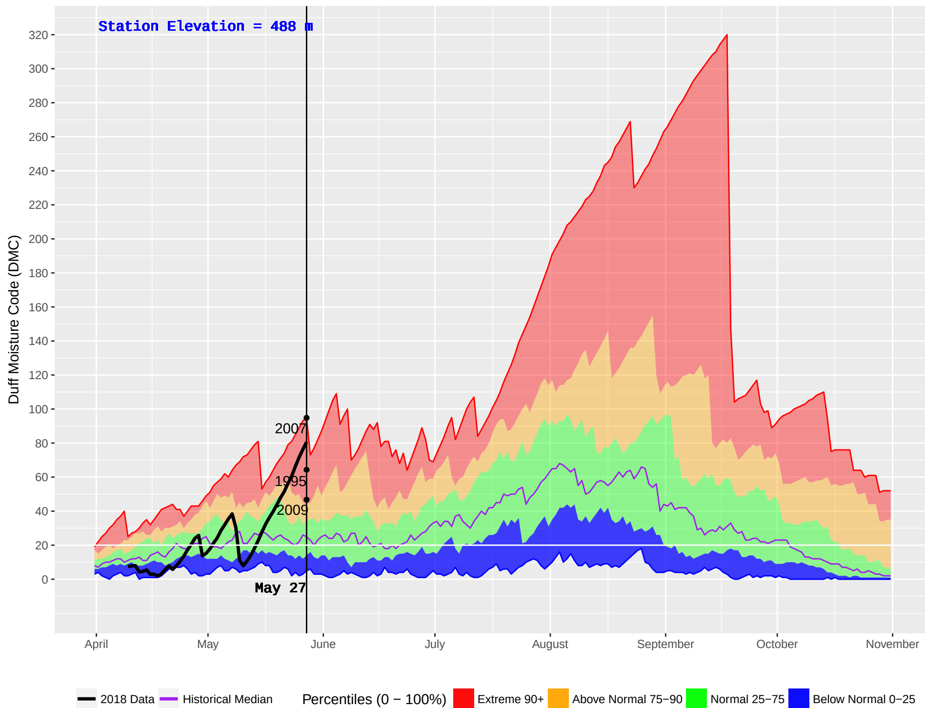
MABEL LAKE 2 (362) : Historical (1987–2016) and Current (2018) Noon Duff Moisture Code (DMC)
